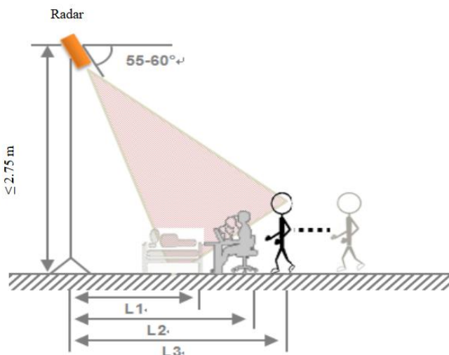
Fig. 7 Look-down mounting
