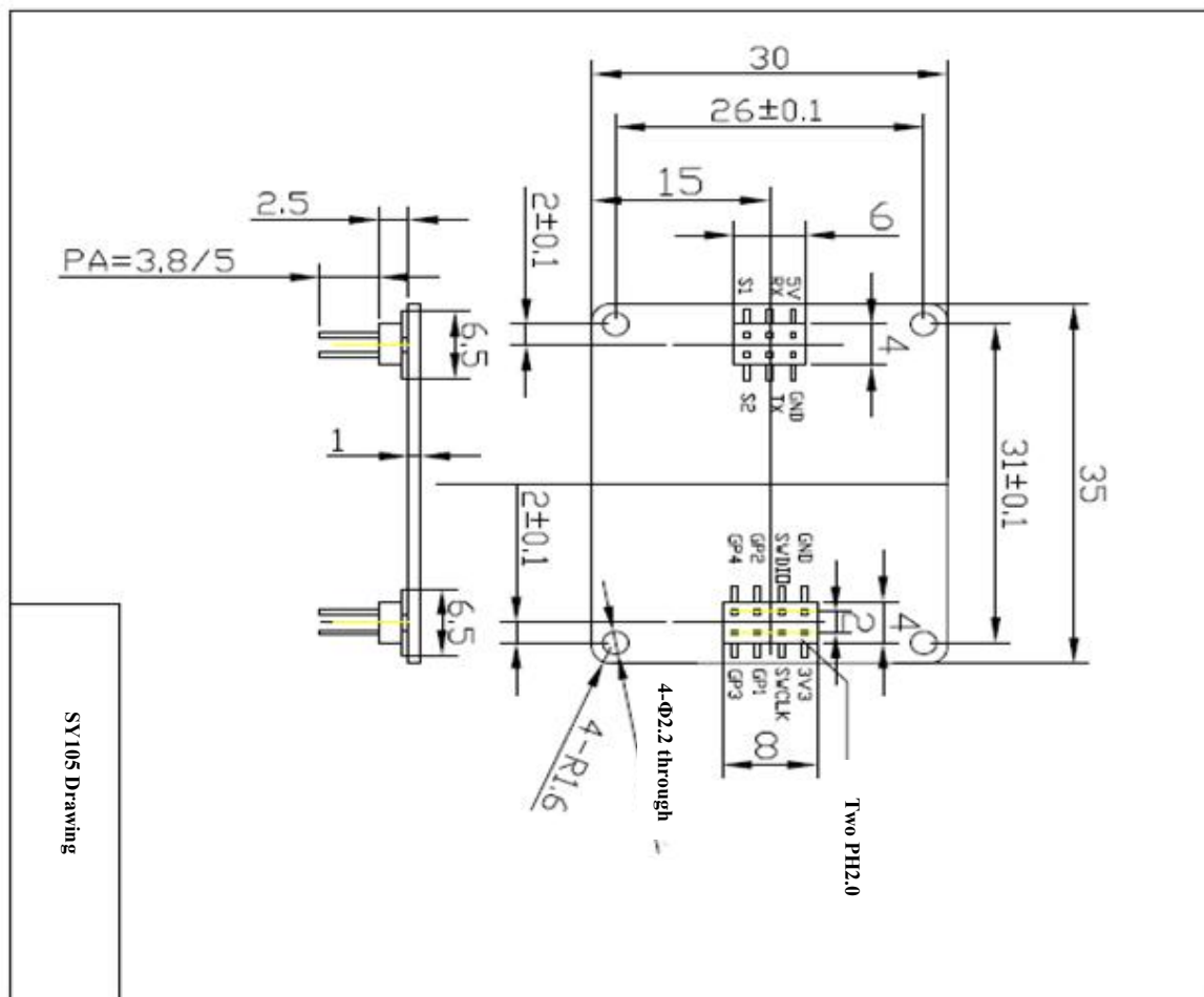
Fig. 2: Schematic diagram for radar module frame
