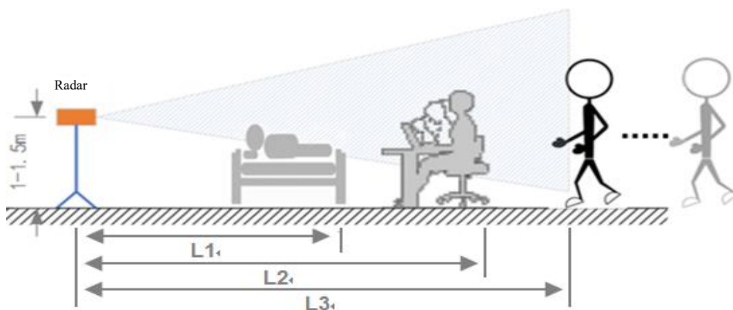
Fig. 6 Horizontal mounting diagram
